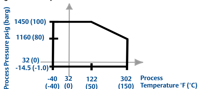
Figure 1. Process pressure
