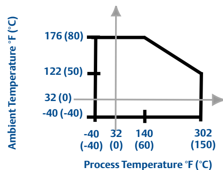
Figure 2. Operating temperatures
